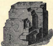
Cubic Cleavage—Galena.
